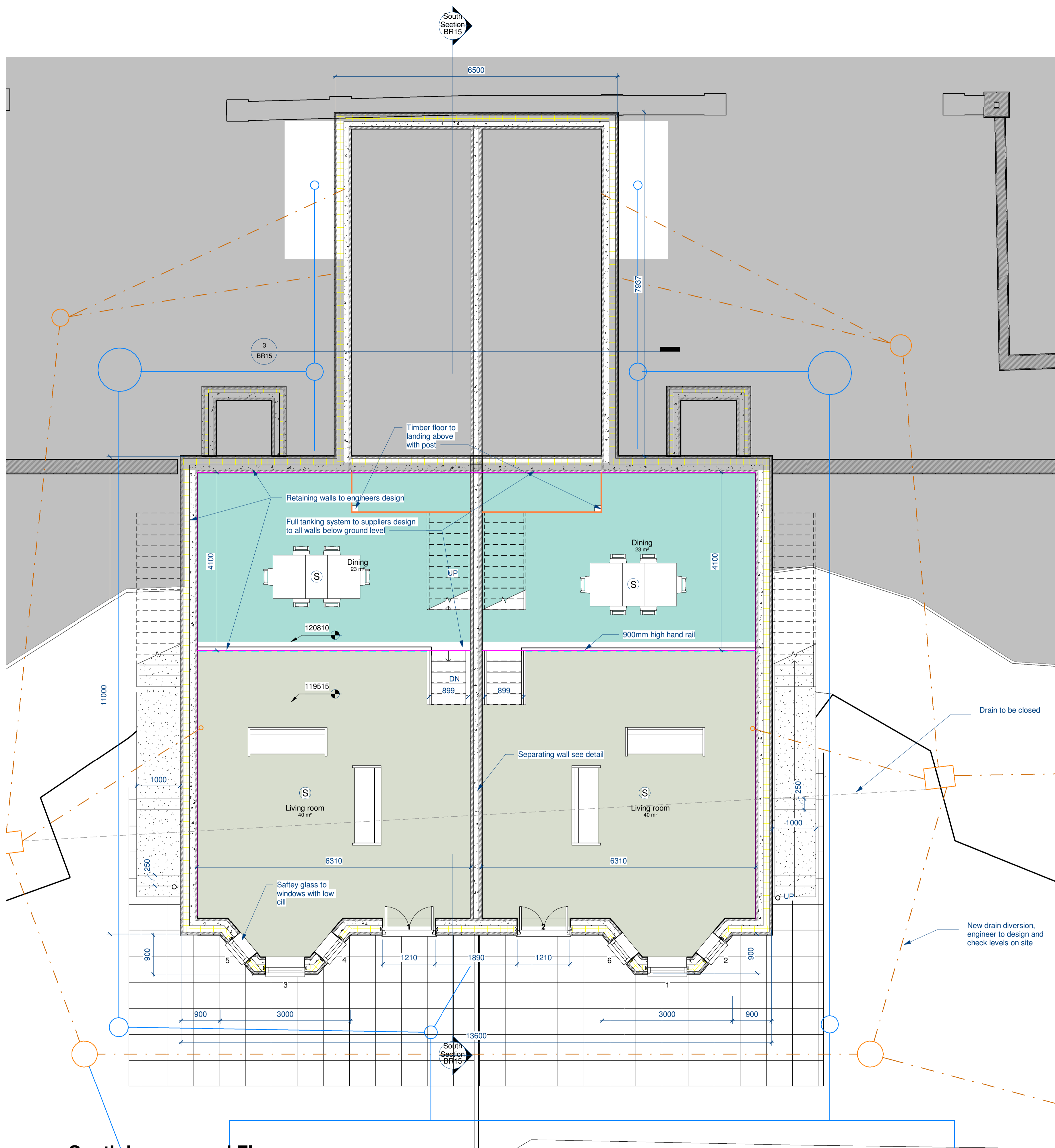
1 South Low ground Floor 1 : 50
