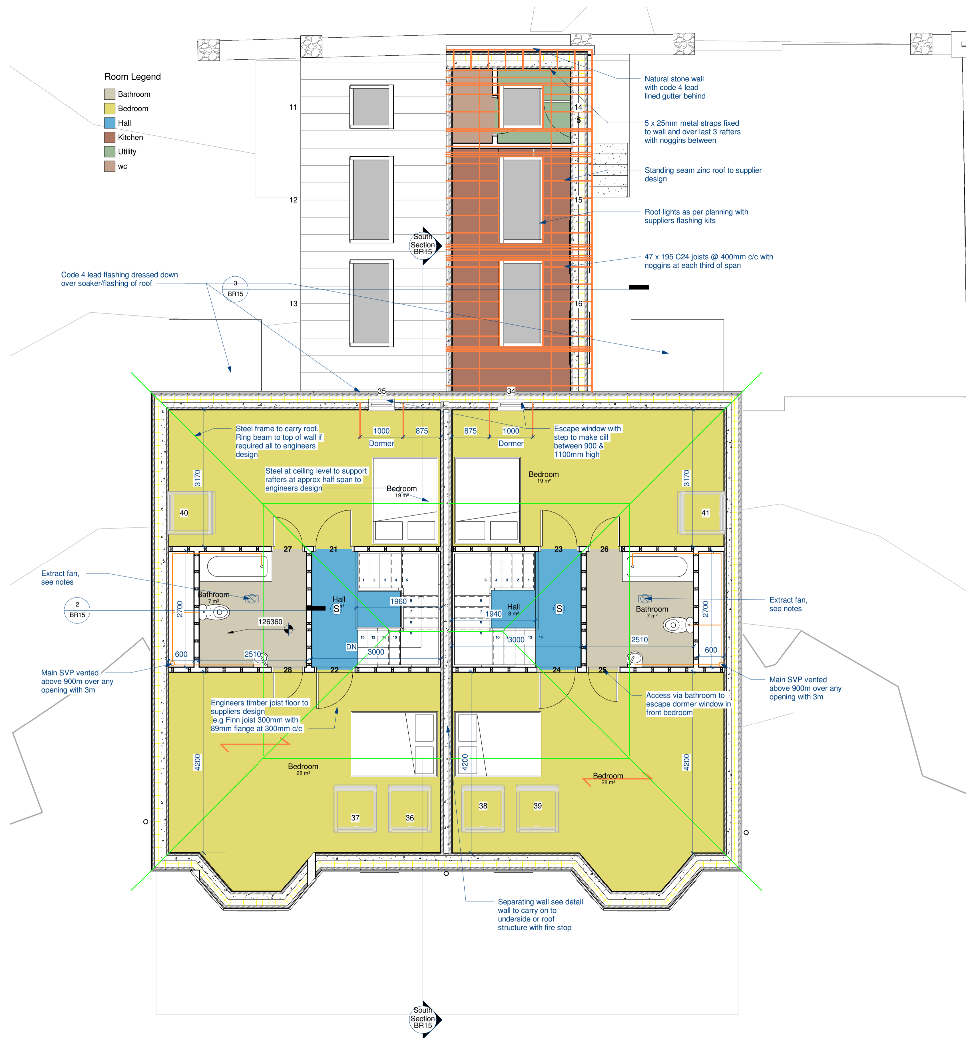
1 South First floor 1 : 50
